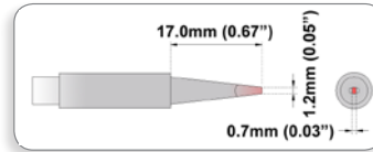
TMT-H-M-1.2D Chisel, 1.2mm (0.47") Equivalent to 900M-T-1.2D
