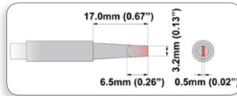
TMT-H-M-3.2D Chisel, 3.2mm (0.126") Equivalent to 900M-T-3.2D
