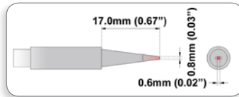
TMT-H-M-0.8D Chisel, 0.8mm (0.032") Equivalent to 900M-T-0.8D
