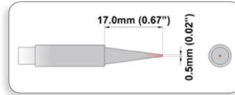
TMT-H-M-B Conical, 0.5mm (0.020") Equivalent to 900M-T-B
